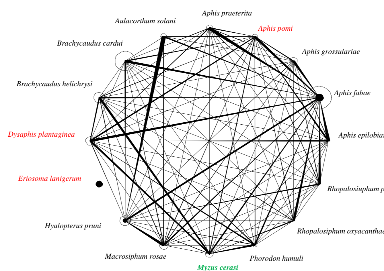
Figure 2. Quantitative parasitoid overlap diagram. The vertices represent aphid species; white circle sizes indicate the relative size of aphid species population; black circle sizes indicate the contribution of the aphid species as a source of its own parasitoids. Polygons between aphid species denote shared parasitoid interaction strength, where the width of the link to each species represents the potential effect derived from another aphid species as a source of parasitoids.
